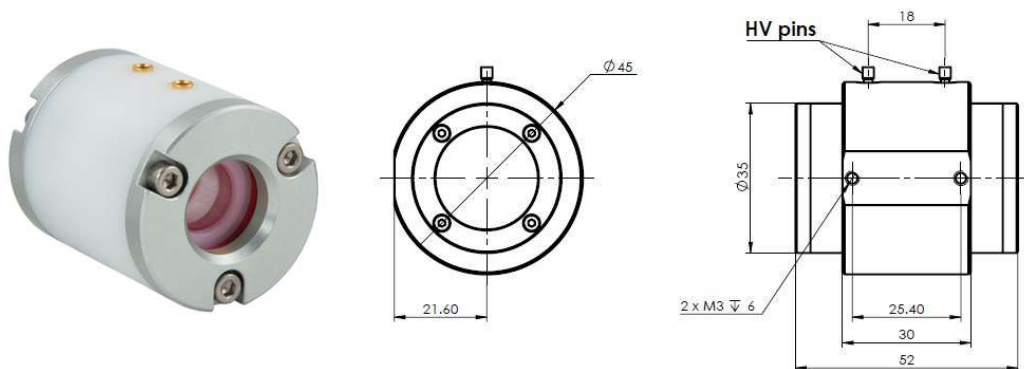
Outline picture and drawing of PC22SR-2/2 DKDP (KD*P) Pockels cell
